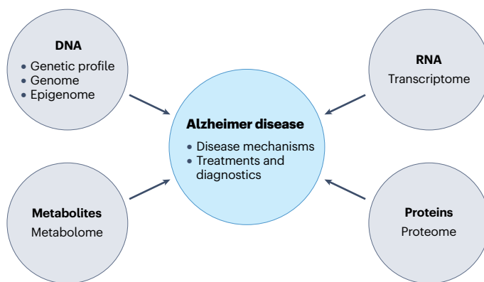
Fig. 6 | An integrated multiomics approach. Integrated multiomics approaches can be used to understand how genetic variation leads to disease, to establish which molecular pathways are altered, and to identify new therapeutic targets and diagnostic approaches. Expression quantitative trait loci (eQTLs) would be generated from each omics layer (gene expression from the transcriptome, protein quantitative traits from the proteome, methylation quantitative traits from the metabolome). These multiomics layers would then be integrated into a systems analysis that includes information on the genome and epigenome, with the goal of furthering understanding of disease mechanisms and developing novel treatments and diagnostics.
