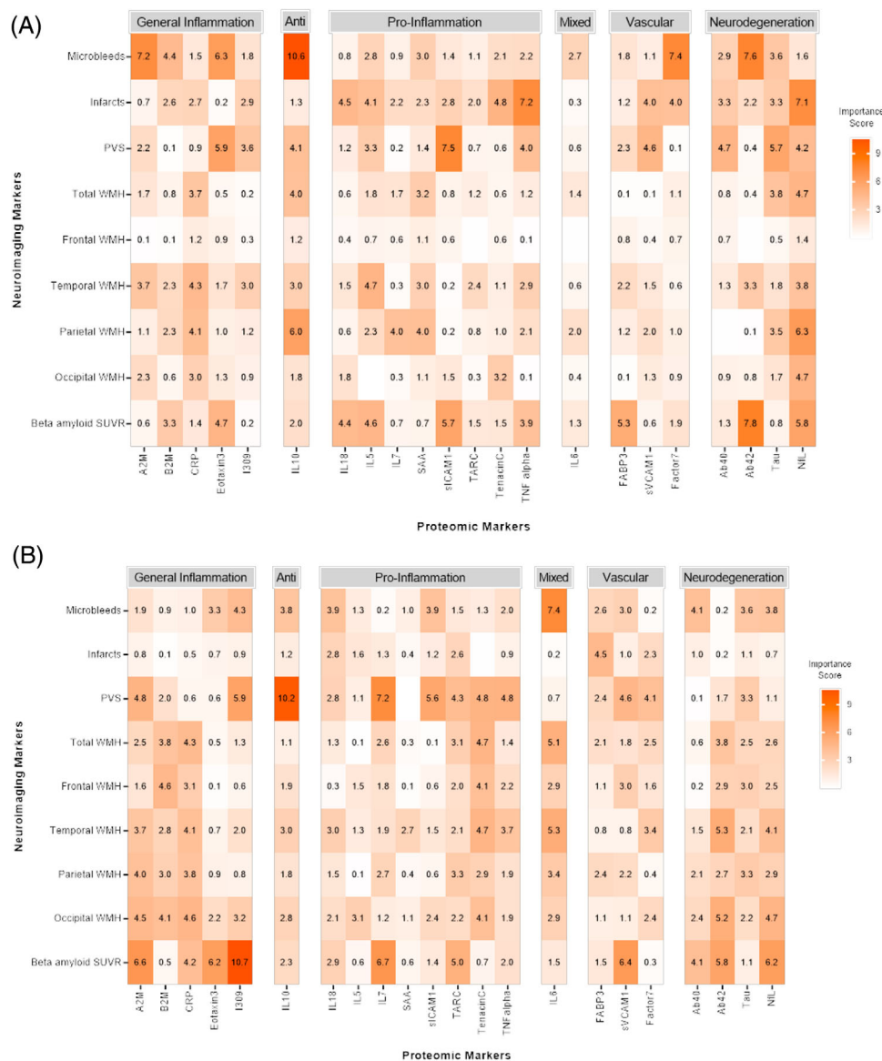
FIGURE 1 Summary of variable important plots. Each row in the heat map represents a separate analysis with numeric variable importance scores displayed and color coded (more saturated reds represent greater relative importance). Top figure (A) includes participants with cognitive impairment and the bottom figure (B) includes those with stable cognitive functioning. Protein markers are grouped by general function, including general inflammation, anti-inflammatory, pro-inflammatory, mixed anti-/pro-inflammatory, vascular, and Alzheimer's disease/neurodegeneration. Anti, anti-inflammation; Mixed, mixed anti-/pro-inflammation
